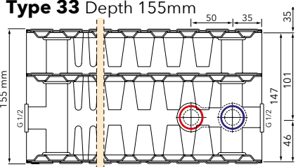
Type 33 Depth 155mm
