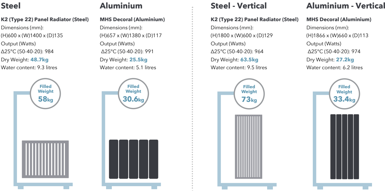
Fig 2. Weight comparison of aluminium and steel radiators
