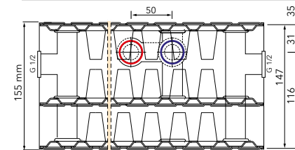
Type 33 Depth 155mm
