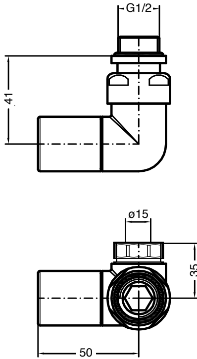
MANUAL VALVE
