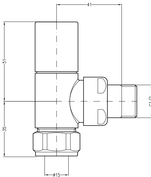
MANUAL VALVE
