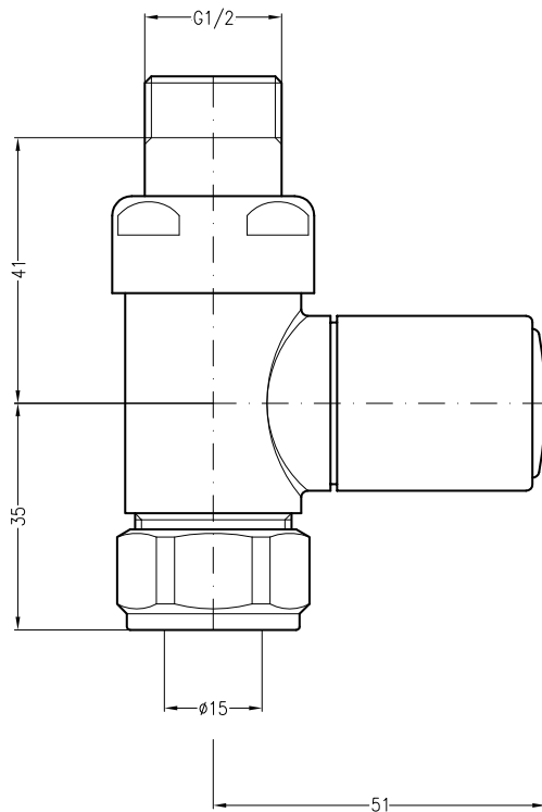
MANUAL VALVE
