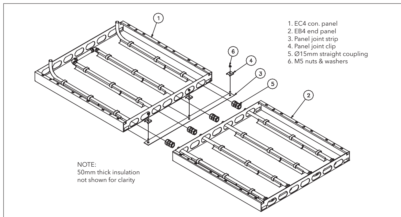
Diagram 1: Moduline Style MCG-4T - typical panel run
