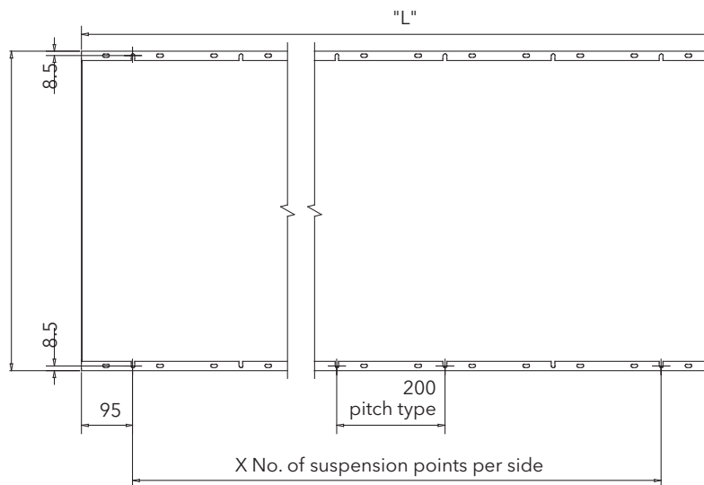
Diagram 3: Typical section detail for installation; Style MCG shown
