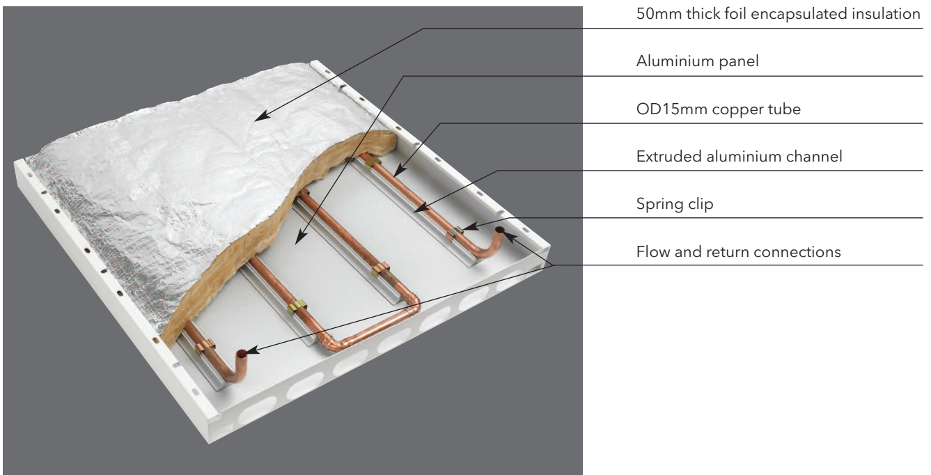
Diagram 5: Moduline Style MCG-4T panel - ED type
